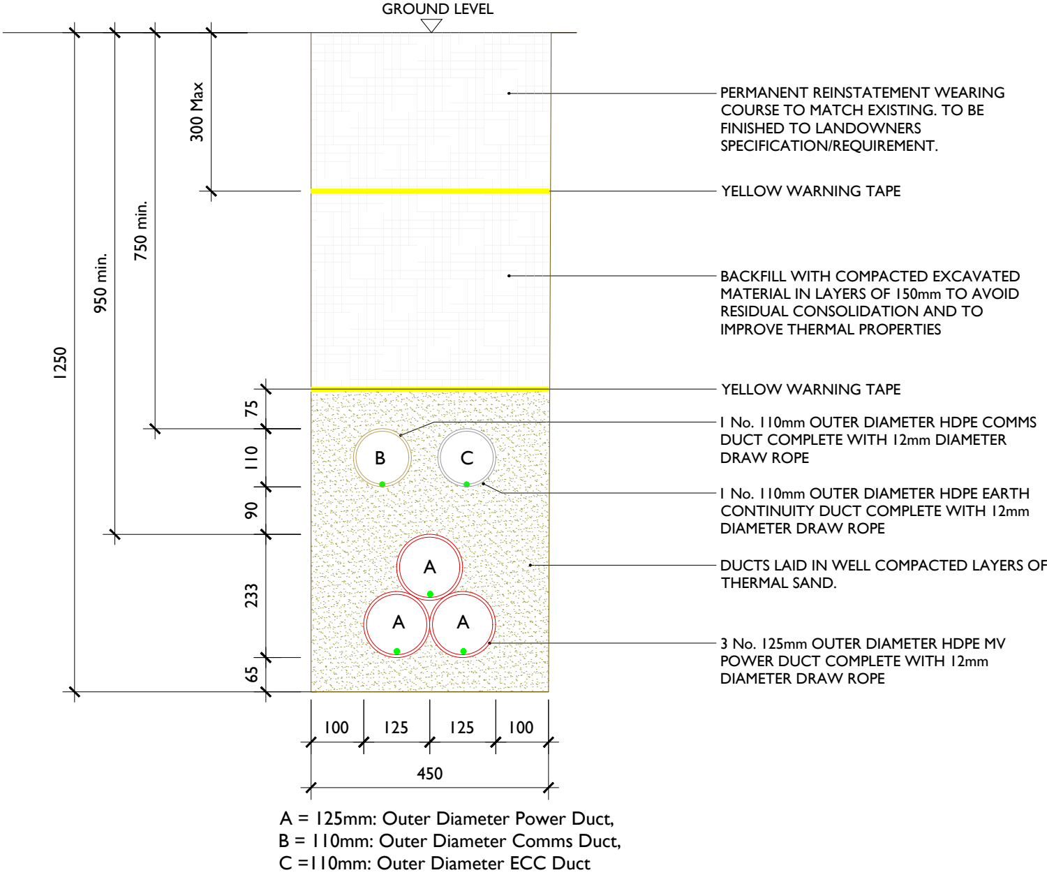
Typical Single Circuit Section Through Grasslands SCALE 1:10
